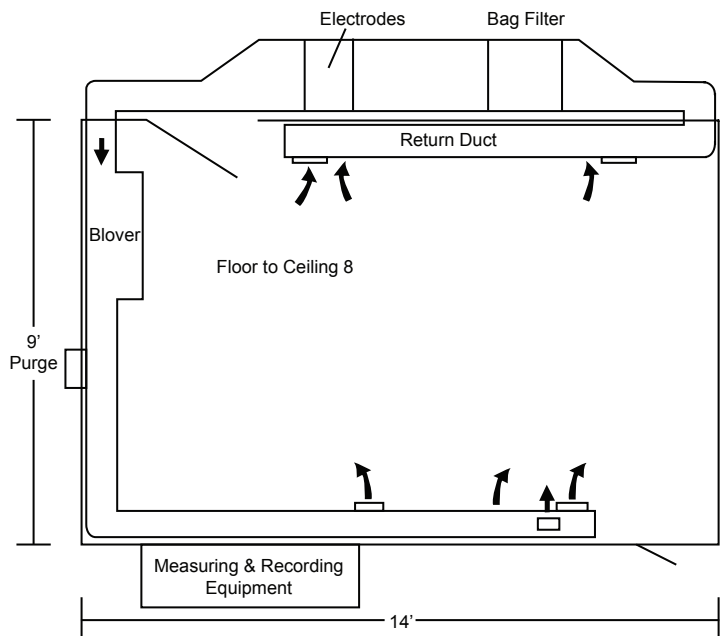
Figure 1. Test Facility Showing Air Handling System
