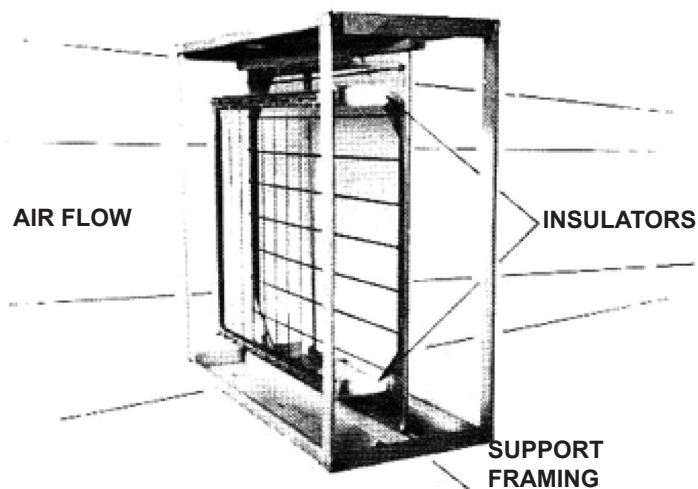
Figure 2. Configuration of electrical field screens
